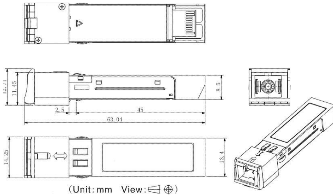
Figure 6. Mechanical Drawing
