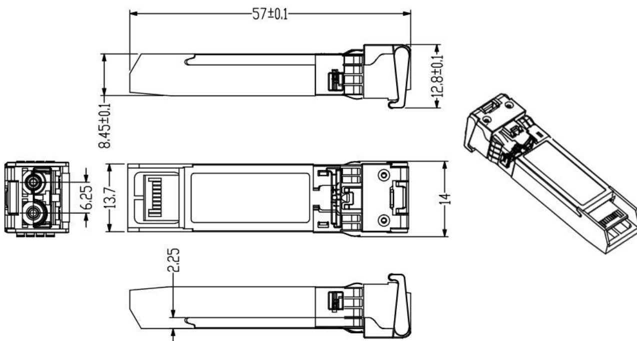
Mechanical Drawing
