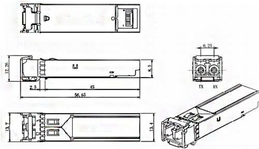
Figure 6. Mechanical Drawing
