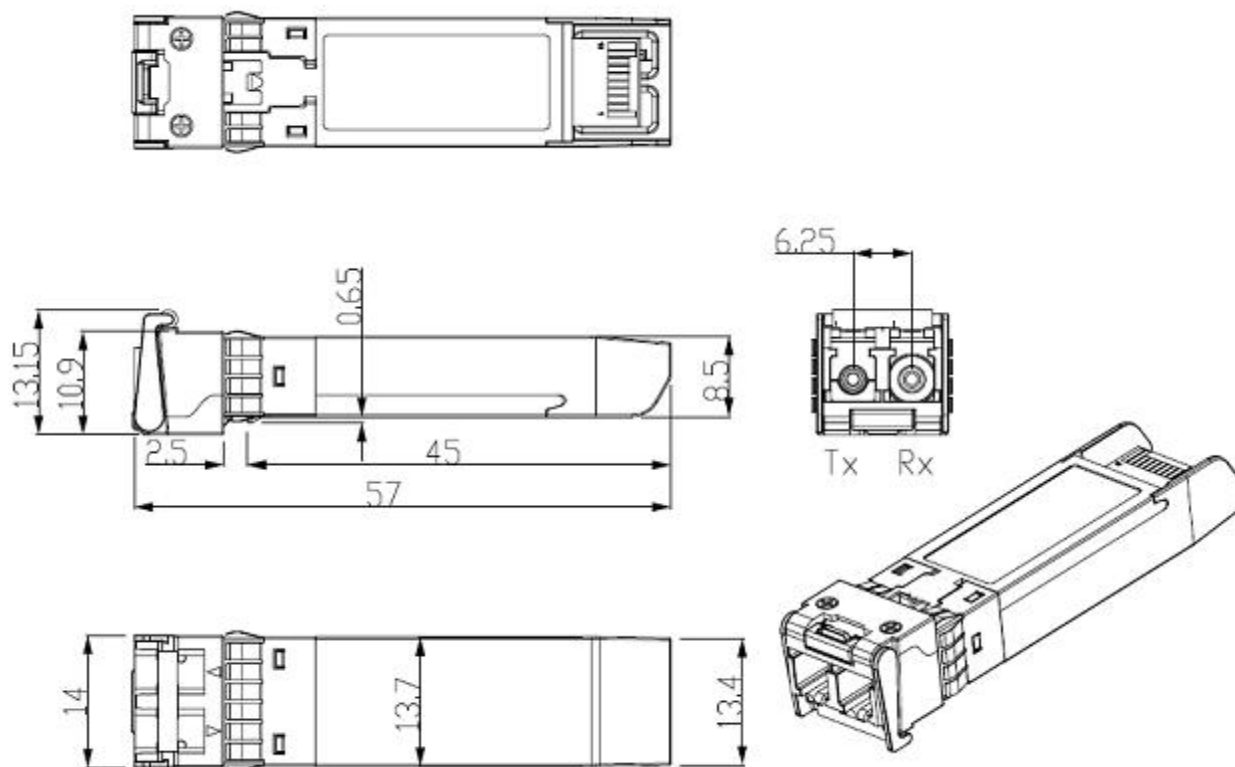
Mechanical Drawing
