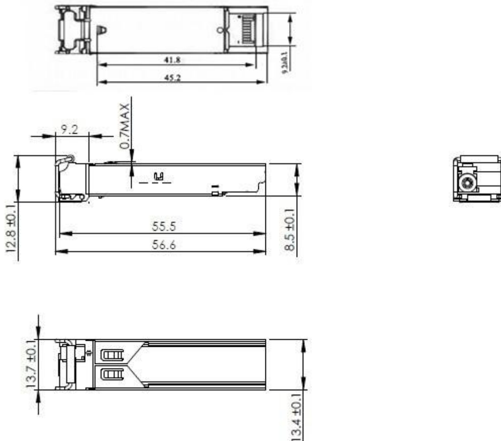
Mechanical Drawing
